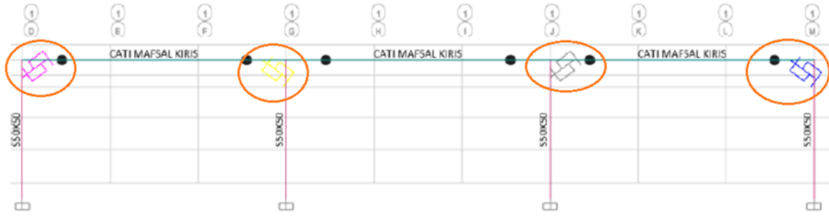
Figure 7: Damper Application in X Direction (Dampers marked with red circles are in diagonal position close to top of the columns and between column and beams).
