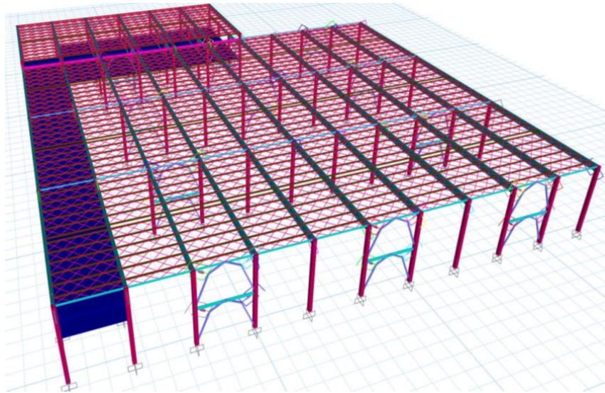
Figure 9: Etabs Model View of Damper Application.
