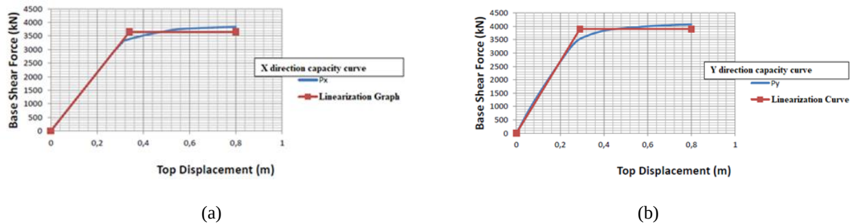
Figure 10: a): X Direction Push Over Capacity Curve b): Y Direction Push Over Capacity Curve
