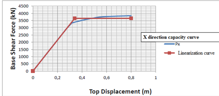
Figure 5: X Direction Capacity Curve
