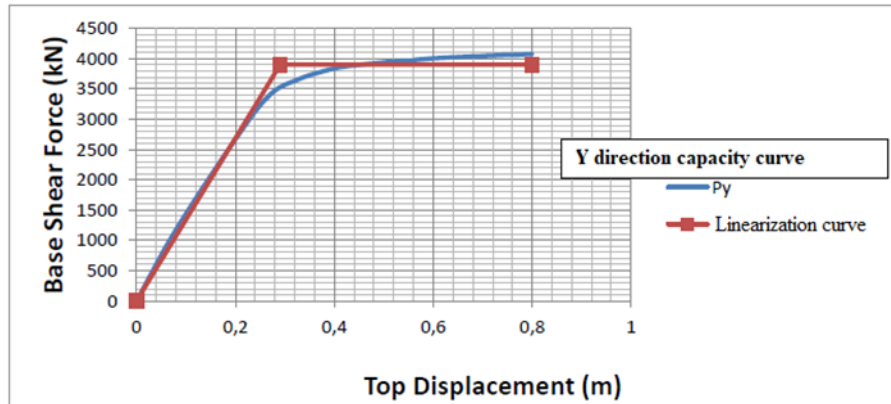
Figure 6: Y Direction Capacity Curve
