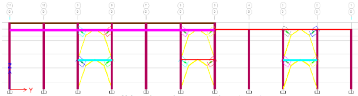
Figure 8: Damper Application in Y Direction (Dampers are in toggle braces)
