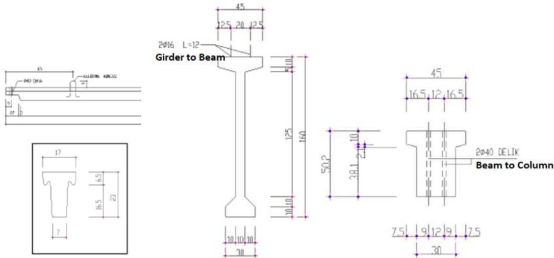
Figure 11: Pin Connection of Girder to Beam and Beam to Column
