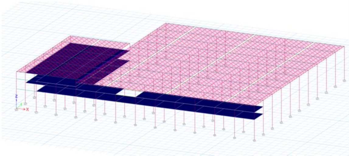
Figure 3: 3-D Etabs model perspective view.
