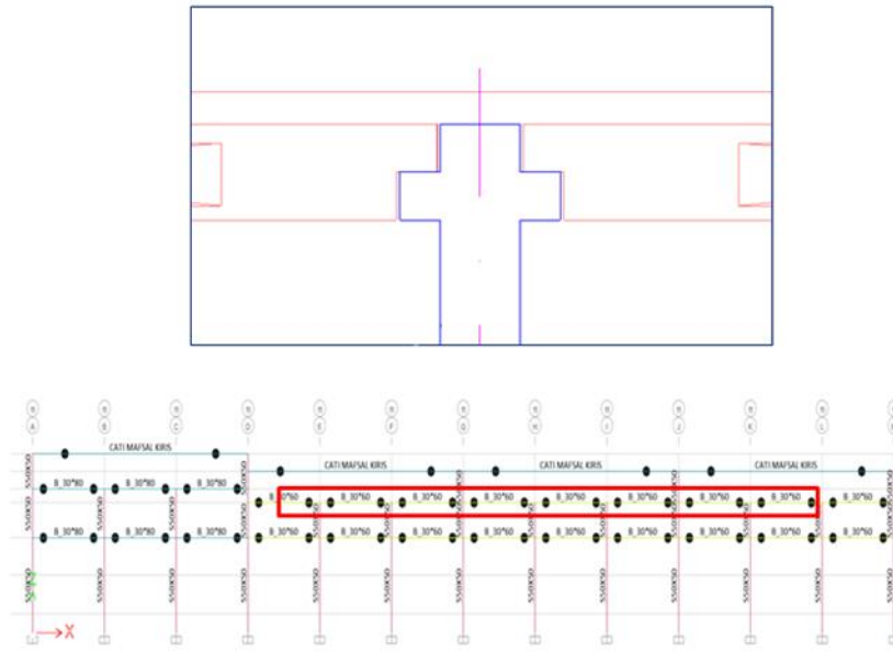
Figure 4: Nonlinear hinge definition for columns and beams
